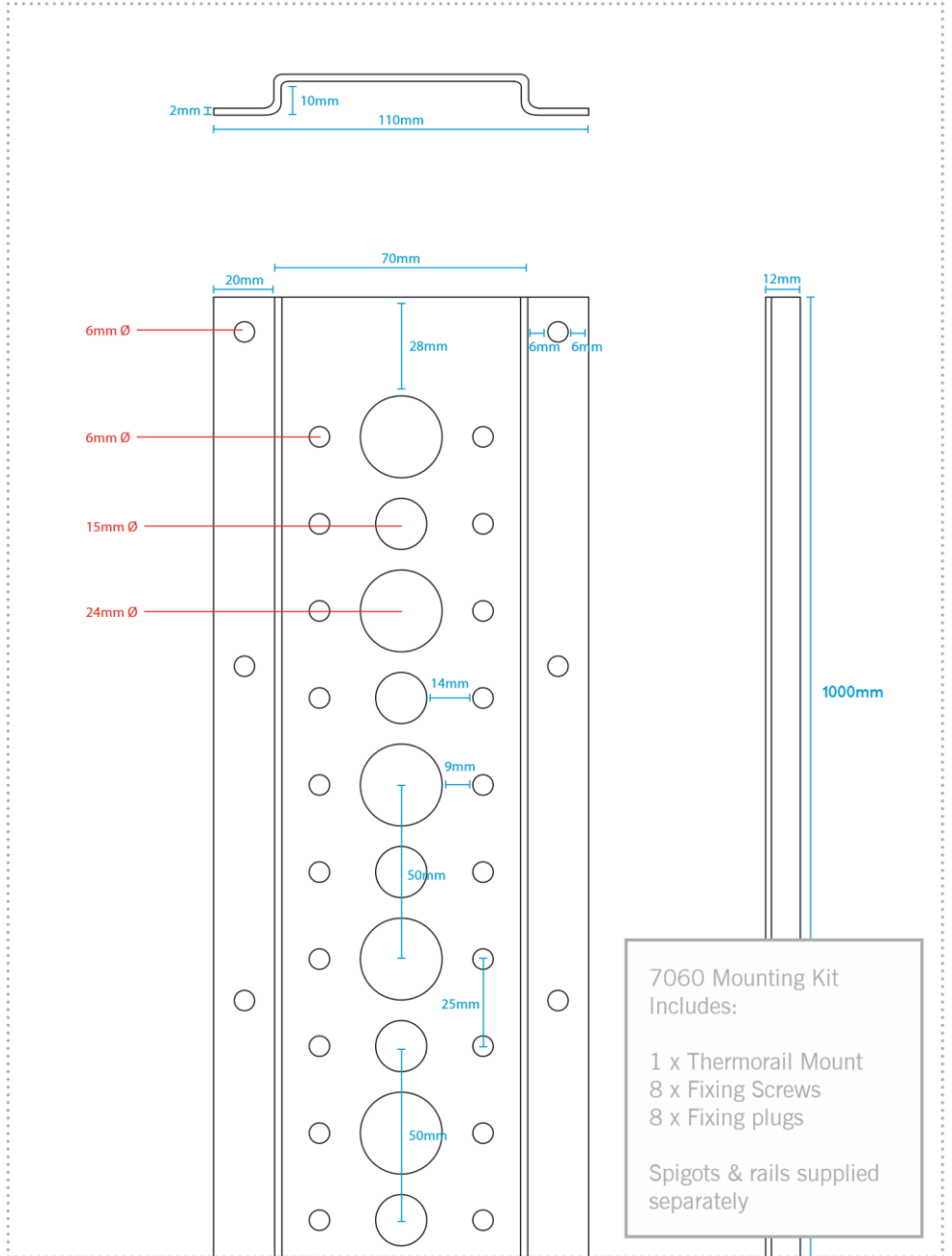
Electric connection cables can be run behind the mounting rail for simple connection.
